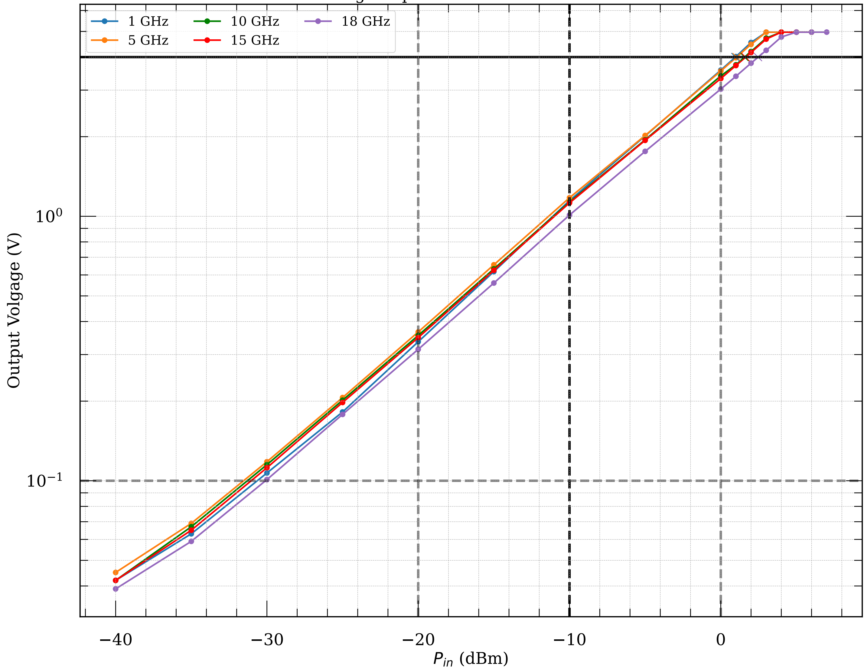
Measured voltage-to-power curve of detector module027v2
